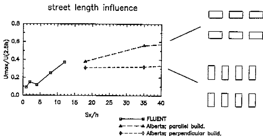
Figure 4.21: Maximum normalized wind speeds U_{max}/U_{2.5h} at street centre line as a function of street length S_x/h . Solid line: FLUENT data for S_y/h \gg 1 , h = 10 m, and z_{o,loc} = 0.03 m. Long dashed line: data of various arrangements (Alberts, 1981) with S_y/h = 2 , h = 9 m and z_{o,loc} = 0.0005 m and buildings parallel to street. Short dashed line: as for long dashed line, but with buildings perpendicular to street.
