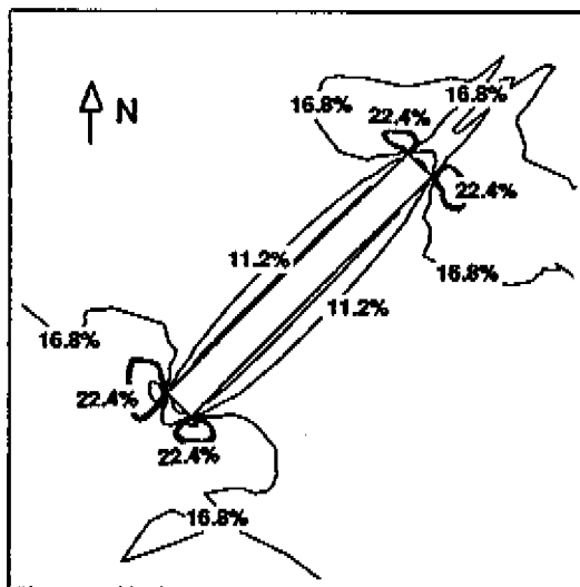
Figure 5.9: Lines of equal discomfort probability around SW-NE oriented building with L, W, H = 15 \times 150 \times 50 m, and z_o = z_{o,loc} = 0.03 m. Contour intervals: 0.25 \cdot P_o , where P_o (thick line) is discomfort probability without building (22.4%).
