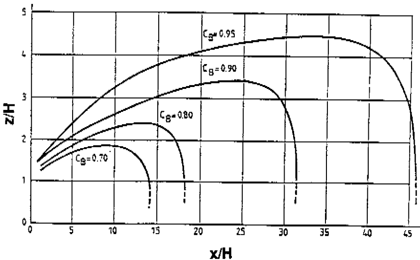
Figure 4.13: Wind speed reduction factor C_B = U(z)/U_0(z) in the far wake of a building (Leene et al, 1990). The graph is valid for normal flow ( 0^\circ ), W/H = 8 , H/z_0 > 30 , C_B > 0.7 , and x/H > 10 . See figure 4.14 for correction graphs for non standard conditions.
