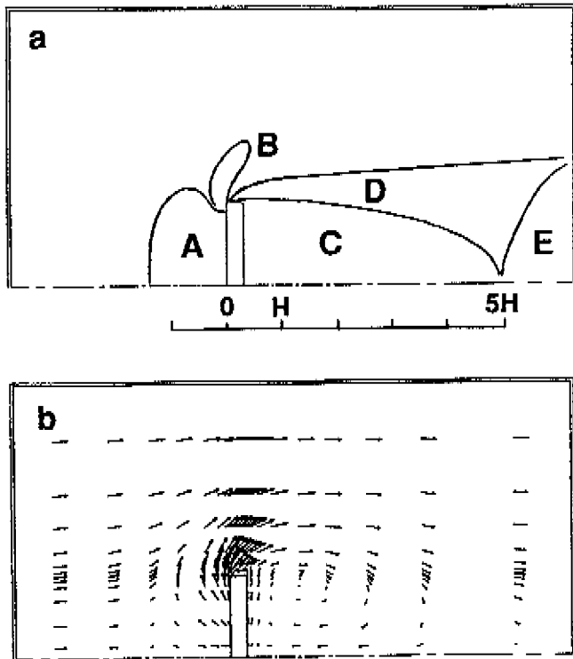
Figure 2.6: Computed time averaged flow properties at pedestrian height (1.75m) around an obstacle with L, W, H = 15, 150, 50\text{m} (normal flow); z_0 = 0.03\text{m} . Because of symmetry, half of the domain is given.
