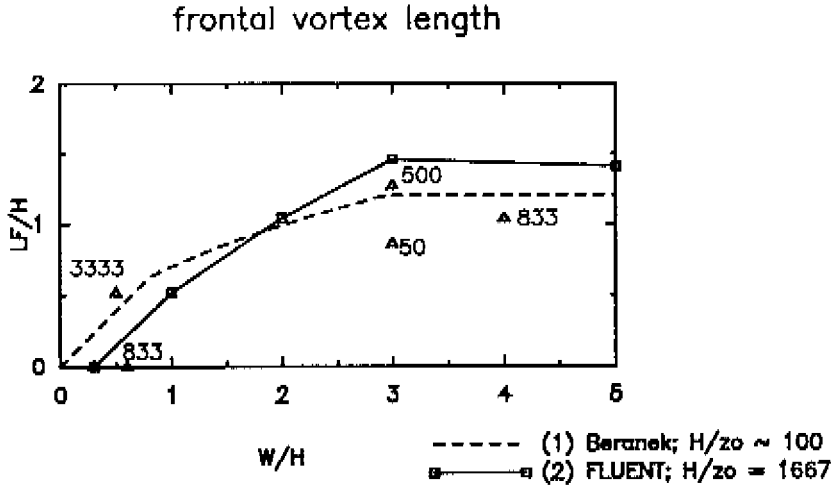
Figure 4.9: Frontal vortex length L_F as a function of W/H . Dashed line (1): flow visualisation data for urban approach flow, followed by about 500 m open terrain (Beranek, 1984). Solid line (2): numerical data for open terrain ( H/z_0 = 1667 ). Triangle points represent additional numerical data ( H/z_0 given in plot).
