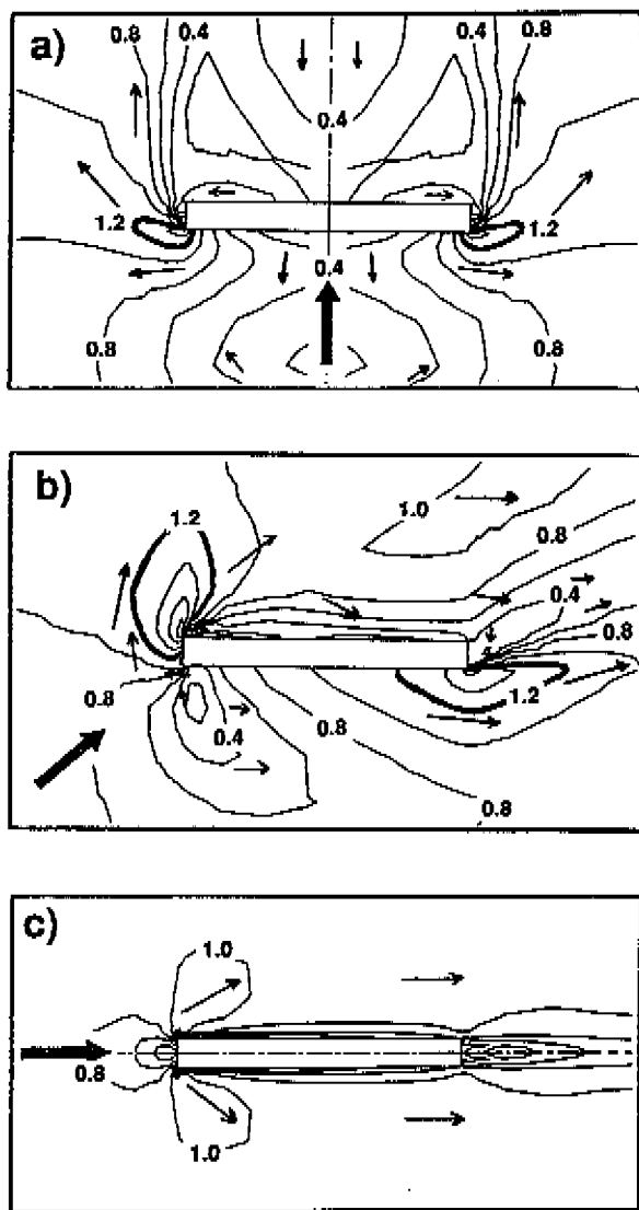
Figure 4.10: Normalized wind speed U/U_0 around building with L, W, H = 15 \times 150 \times 50 m and z_o = z_{o,loc} = 0.03 m, showing location, dimensions and shape of corner streams. U_o/U_{Ho} = 0.55 . Contour intervals: 0.2; thick line: U/U_0 = 1.2 . See fig. 2.6-2.8 for vector plots and flow patterns.
