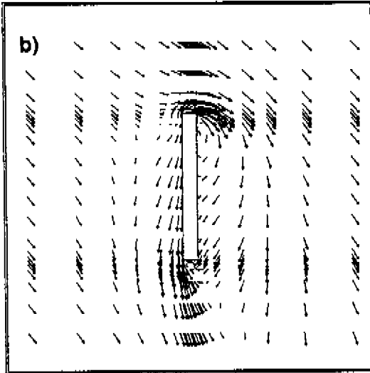
Figure 7.5: Time averaged pedestrian level flow pattern around a building of 15x150x50 m (thickness, width, height) together with location of high wind speed regions (corner streams).
