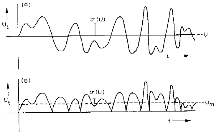
Figure 2.11: Instantaneous streamwise velocities (a), compared with 'hot wire results' (b). Only absolute values of U(t) are measured in (b). U and \sigma_u denote real mean velocity and standard deviation, U_m and \sigma_{um} 'measured' values.
