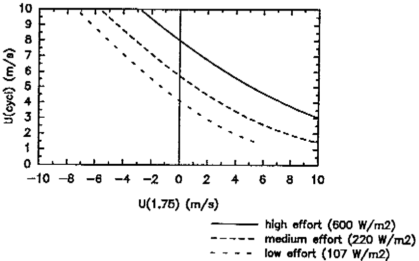
Figure 3.2: Maximum cycling speed (uncertainty \sim 25\% ) as a function of wind speed. Negative x-axis: tail winds; positive x-axis: head winds. Base metabolic rate 70 \text{ W/m}^2 . All work is used to overcome the air resistance. Upper line: M/A_{Du} = 600 \text{ W/m}^2 ; maximum for well trained people Middle line: M/A_{Du} = 220 \text{ W/m}^2 ; maximum for untrained people Lower line: M/A_{Du} = 107 \text{ W/m}^2 ; little effort required
