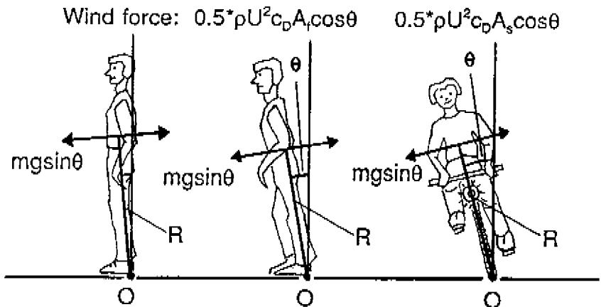
Figure 3.1: Force moments due to wind force and gravitational force on people standing right up, people leaning into the wind, and a cyclist leaning into the wind.
