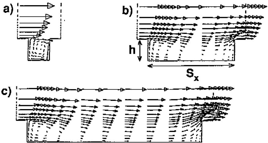
Figure 2.9: Computed flow patterns (2 dim.) typical of flow regimes in building groups. a) S_x/h = 1 skimming flow b) S_x/h = 4 wake interference flow c) S_x/h = 8 isolated roughness flow
