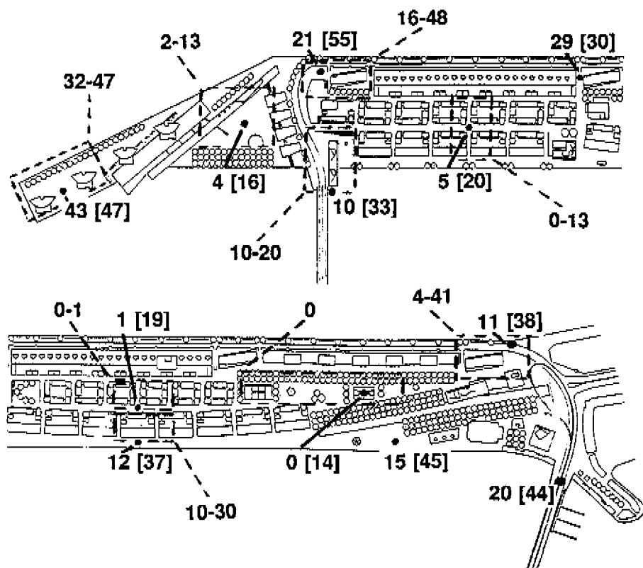
Figure 6.8: Discomfort probability (in days per year) for the 12 points of figure 6.7b and for some areas (dashed boxes) as determined by IMET-TNO (Harst, 1992). See table 6.2 for criteria. Desk estimates are given in square brackets.
