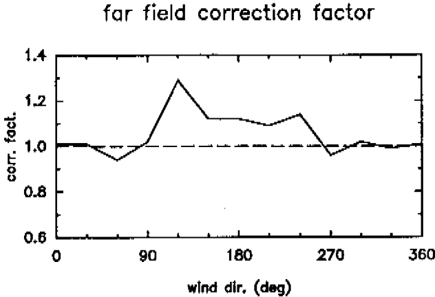
Figure 6.10: Ratio of present reference wind speed and TNO data as a function of wind direction \theta . Reference speed is given at turntable edge (863 m from centre of island) and at 26 m height. The ratio can be considered as correction factor for TNO data.
