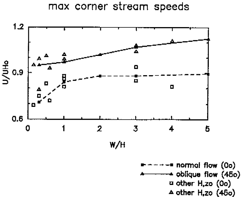
Figure 4.12: Maximum corner stream wind speeds U/U_{Ho} as a function of W/H for two approach flow angles: 0^\circ (lower curve) and 45^\circ (upper curve). Further data: H = 50 m; L = 15 m; z_o = 0.03 m. For large W/H , blockage effects (up to 2.5%) result in slight overestimation of U/U_{Ho} .
