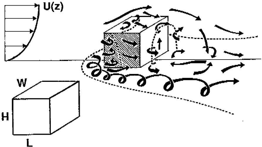
Figure 2.5: Flow field around an obstacle which is immersed in the atmospheric boundary layer, together with notation definition.
