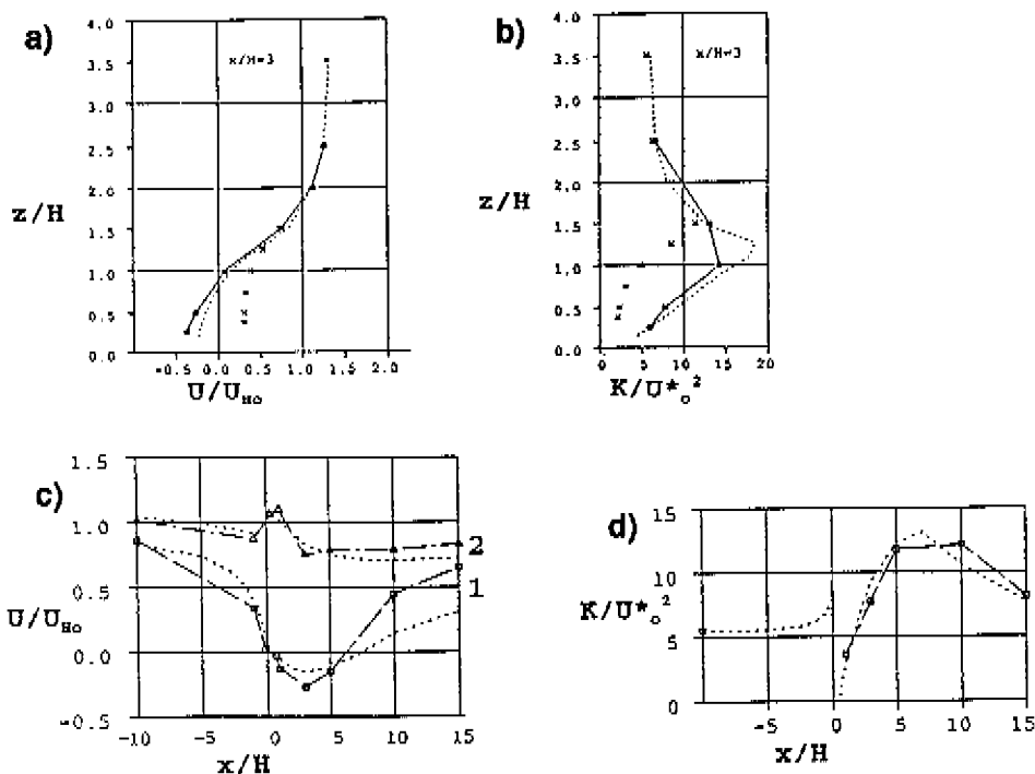
Figure 2.14: Normalized mean velocity U/U_{H_0} and normalized turbulent kinetic energy K/U_{*0}^2 behind single wide block (normal flow: \mathcal{O}^{\circ} ). Cross points: hot wire results; square points / solid line: LDA results; dotted line: FLUENT results.
