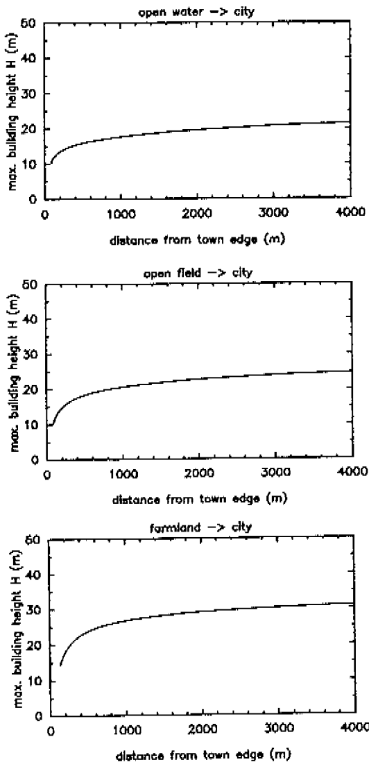
Figure 7.7: Maximum building height for which wind climate is acceptable at all nearby locations. The x-axis gives distance to town edge in metres. Area below solid line is acceptable for 'walking fast' and 'strolling' activities. Valid for all building orientations.
