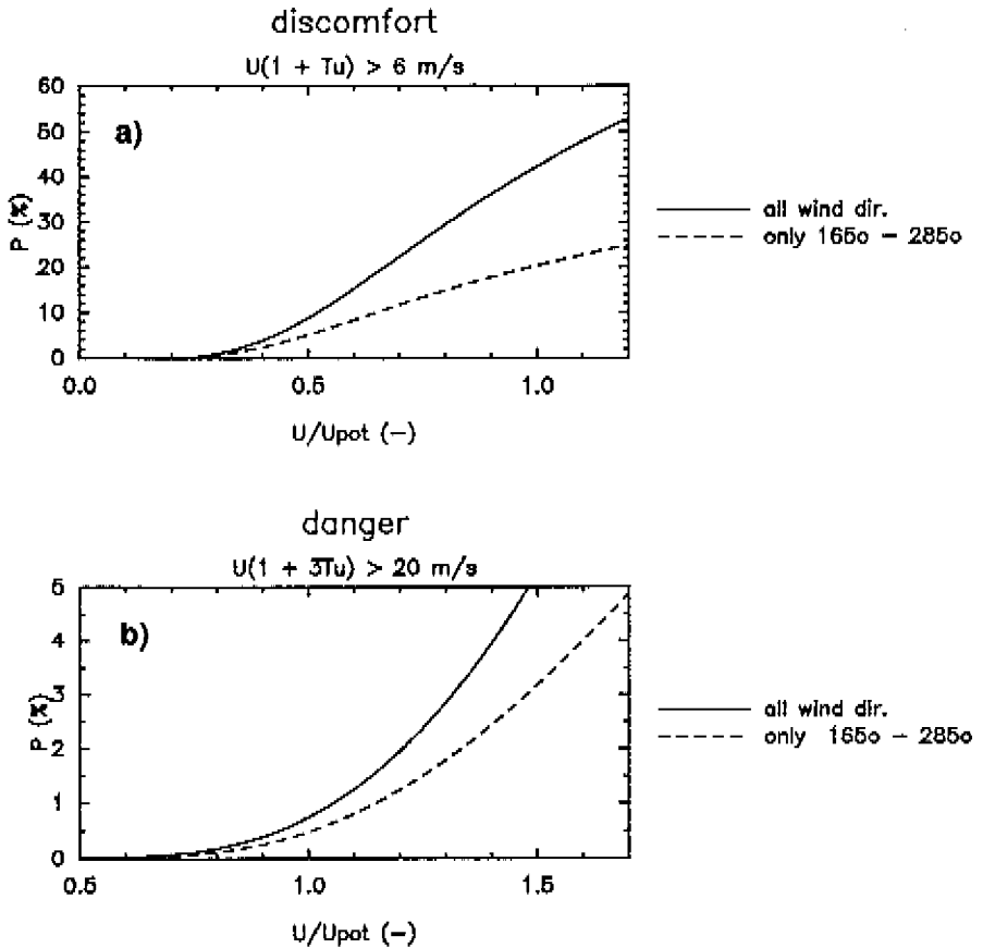
Figure 5.1: Discomfort and danger probability as a function of direction independent wind amplification factor \gamma ( U/U_{pot} ). Solid line: total probability. Dashed line: contribution of southwesterly wind directions ( \theta between 165^\circ and 285^\circ ). Climate statistics: Amsterdam airport (Troen et al, 1989). Standard deviation \sigma_u is equal to airport value.
