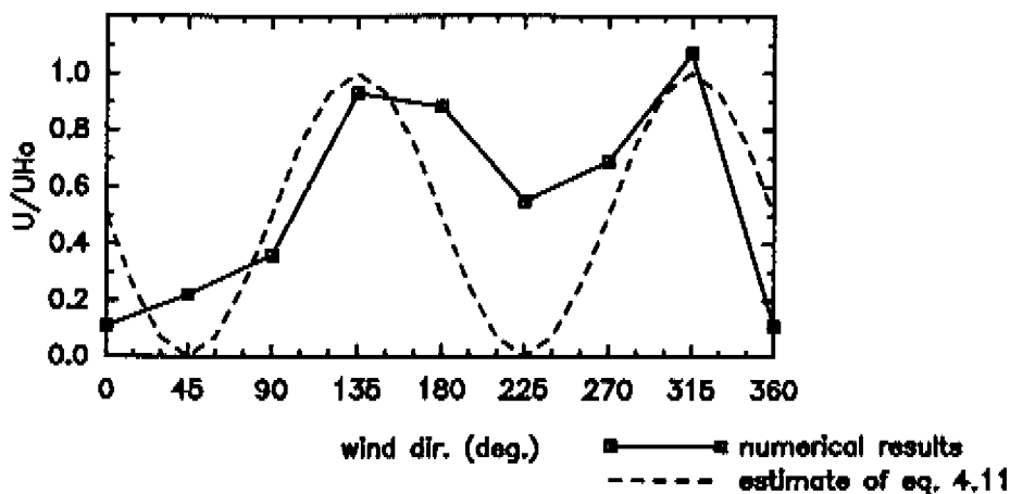
Figure 4.31: Wind conditions at SW corner of E-W oriented building ( L, W, H = 15 \times 150 \times 50 m; z_o = z_{o,loc} = 0.03 m): U/U_{Ho} as a function of \theta . Solid line: present numerical data. Dashed line: estimate of eq. 4.11.
