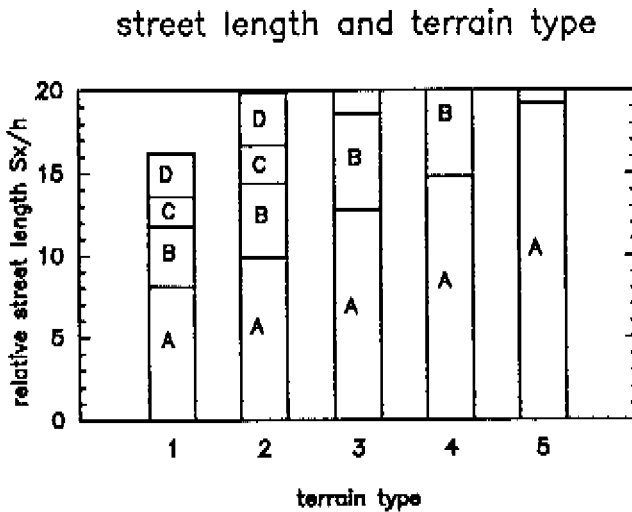
Figure 7.2: Relative street length (street length divided by building height: S_x/h ) for which wind climate is acceptable. The x-axis gives 5 terrain types as given in table 7.1. Street orientation is SW-NE. A, B, C, D indicate allowed types of activities: long stay, short stay, strolling, walking fast (table 7.2).
