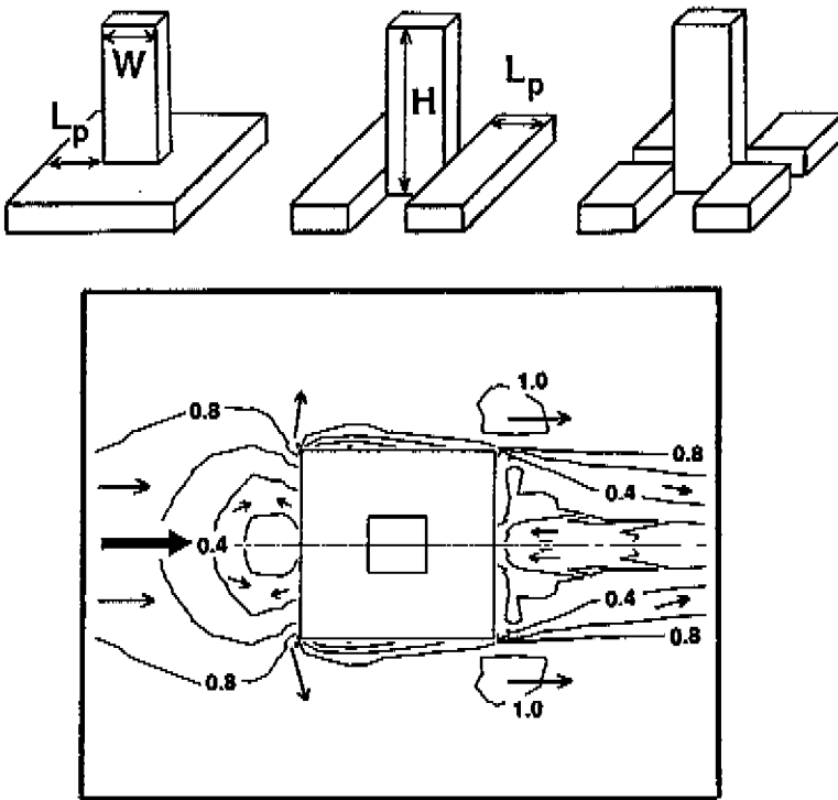
Figure 4.25: Building with podium shaped extensions: geometry and flow field
