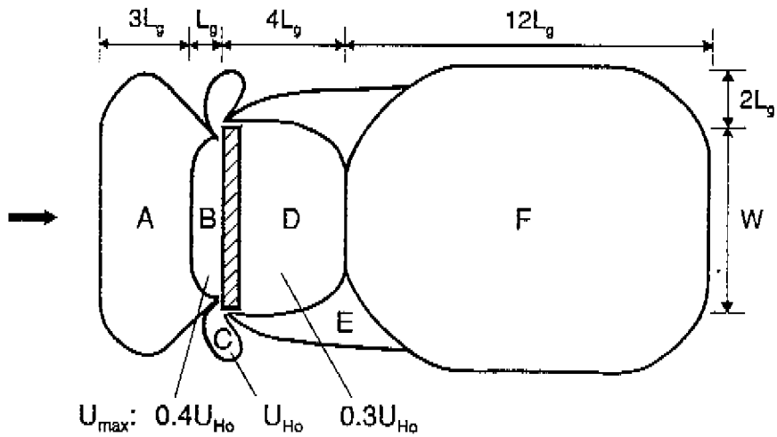
Figure 4.8: Influence area and flow zones around a building (normal flow; 0_0 ). Dimensions (mainly from numerical data discussed later) are given as a multiple of the geometrical influence scale L_g (eq. 4.8). Maximum wind speeds are given as well. Flow zones given are: upstream retarded zone (A), frontal vortex (B), Corner streams (C), recirculation zone (D), shear layers (E), far wake (F).
