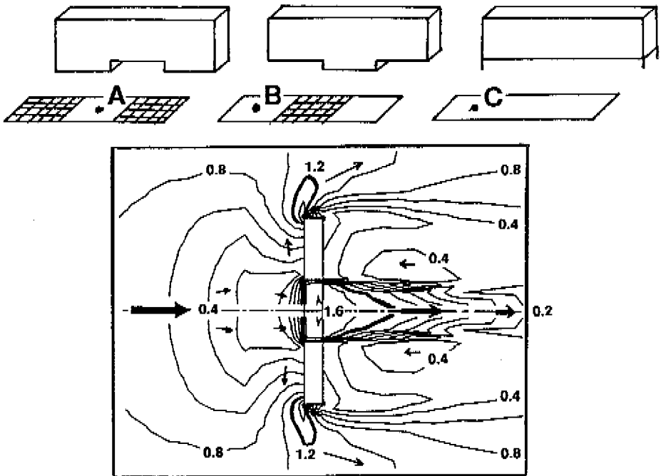
Figure 4.23: Building with ground level gap(s): classification and flow field a) Examples of buildings with ground level gaps; wind speeds for points A, B, C are given in table 4.7 b) Normalized wind speed U/U_0 around building with L, W, H = 15 \times 150 \times 50 m. Further data: normal flow ( 0^\circ ); gap width W_{gap} = 50 m; gap height H_{gap} = 10 m; z_o = z_{o,loc} = 0.03 m; U_o/U_{Ho} = 0.55 . Contour intervals: 0.2; thick line: U/U_0 = 1.2 .
