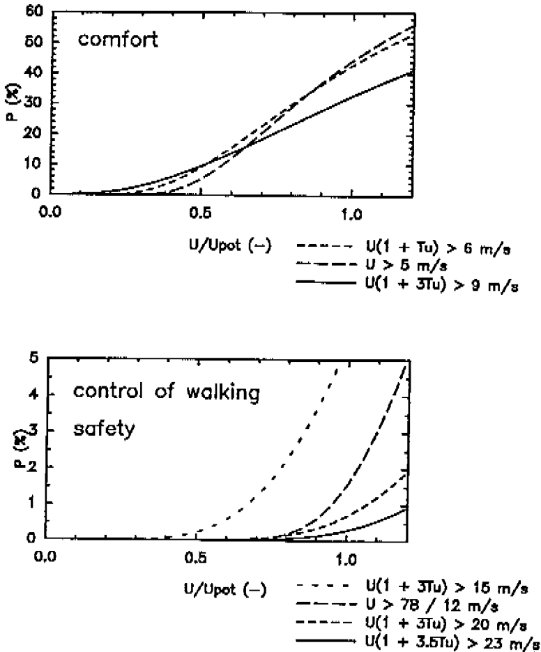
Figure 3.4: Percentage of time that comfort and safety requirements are not met as a function of direction independent wind amplification factor \gamma ( U/U_{pot} ). Climate statistics: Amsterdam airport (Troen et al., 1989).
