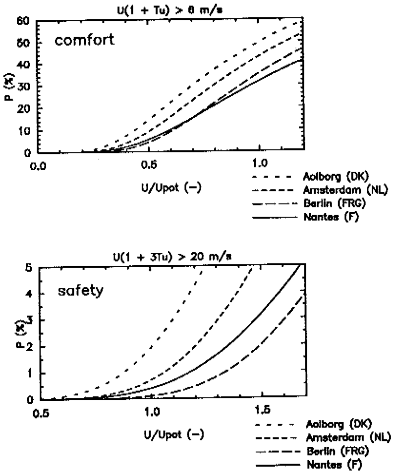
Figure 3.6: Discomfort and danger probability (%) as a function of direction independent \gamma ( U/U_{pot} ) for some European stations: Amsterdam (NL), Aalborg (DK), Berlin (FRG) and Nantes (F).
