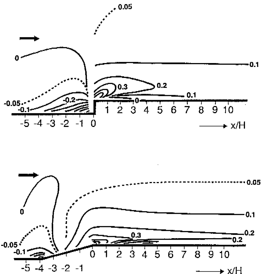
Figure 4.5: Fractional speed up factor \Delta S as a function of x/H and z/H over a cliff escarpment and over a gentle sloping ramp (after Bowen, 1977).
