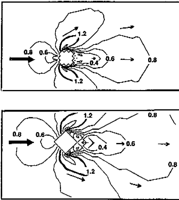
Figure 4.27: Relative wind speed U/U_0 around 15 \times 15 \times 50 m ( L, W, H ) building for oblique flow ( 45^\circ ); z_0 = z_{0,loc} = 0.03 m; U_0/U_{H0} = 0.55 . Contour intervals: 0.2; thick line: U/U_0 = 1.2 . Upper plot: with stepped corners; lower plot: without stepped corners. Note reduction in 'effective' (lateral) building width and in corner stream and wake dimensions in upper plot.
