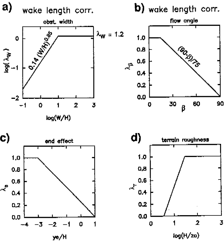
Figure 4.14: Correction graphs for wake length of figure 4.13 (after Leene et al, 1990). a) Effect of relative obstacle width b) Effect of approach flow angle c) Effect of obstacle ends d) Effect of ratio of building height and terrain roughness H/z_0 (use of graph not recommended for H/z_0 < 20 )
