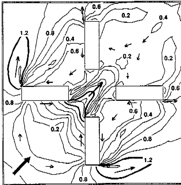
Figure 4.20: Normalized wind speed U/U_0 for a cross ('+') shaped building arrangement (oblique flow; 45^\circ ). Building dimensions are 15 \times 50 \times 50 m ( L, W, H ); S_x = S_y = 50 m; roughness length z_0 = z_{0,loc} = 0.03 m; U_0/U_{H0} = 0.55 . Contour intervals: 0.2; thick line: U/U_0 = 1.2 .
