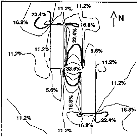
Figure 5.10: Lines of equal discomfort probability around N-S oriented group of shifted buildings with L, W, H = 15 \times 50 \times 50 m, S_z = 20 m, D_y = -50 m, and z_o = z_{o,loc} = 0.03 m. Contour intervals: 0.25 \cdot P_o , where P_o (thick line) is discomfort probability without building (22.4%).
