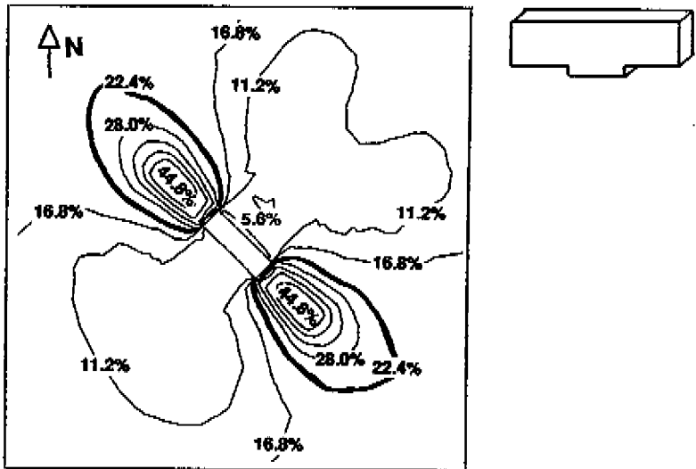
Figure 5.8: Lines of equal discomfort probability around NW-SE oriented building with L, W, H = 15 \times 150 \times 50 m and two corner gaps with H_{gap} = 10 m, W_{gap} = 50 m, and z_o = z_{o,loc} = 0.03 m. Contour intervals: 0.25 \cdot P_o where P_o (thick line) is discomfort probability without building (22.4%).
