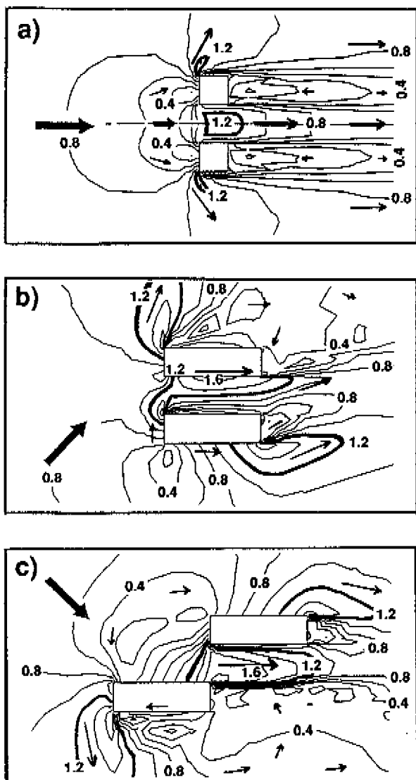
Figure 4.19: Normalized wind speed U/U_0 for different arrangements of parallel buildings. Roughness length z_o = z_{o,loc} = 0.03 m; U_o/U_{Ho} = 0.55 . Contour intervals: 0.2; thick line: U/U_0 = 1.2 .
