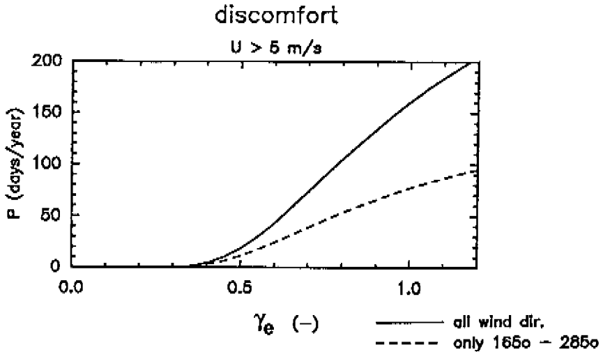
Figure 6.2: Discomfort probability in terms of days (24 h) per year as a function of direction independent wind amplification factor \gamma ( \gamma_e ). Solid line: total probability. Dashed line: contribution of southwesterly wind directions ( \theta between 165^\circ and 285^\circ ). Climate statistics: Amsterdam airport (Troen et al, 1989).
