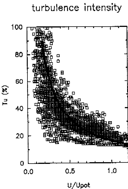
Figure 4.15: Numerical estimate of turbulence intensity T_u (about 20000 data points) as a function of wind amplification factor \gamma . The estimate is made for isolated buildings and for z_0 = 0.03 m. The standard relative error in a constant \sigma_u approximation is 15%.
